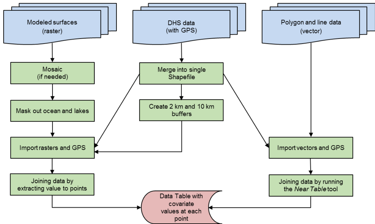
Figure 1: Conceptual framework of the covariate extraction process.
