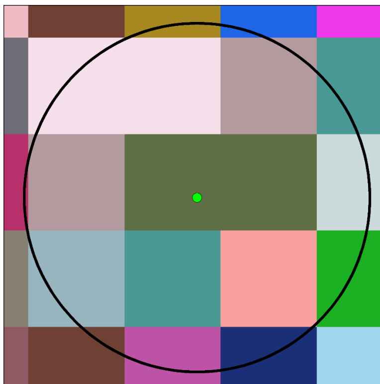
Figure 2: A 10-kilometer buffer around a DHS cluster location
